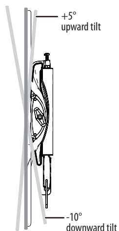
SIDE VIEW - TILT
