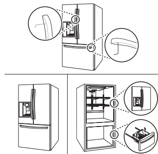
Disassembling/Assembling
