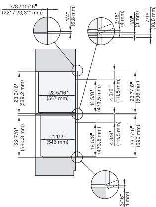
DGC6x6x(AM)+EBA6808, H6S60B+EBA6808, H6x60BP+EBA6808, (DGC786x, H7x6xBP)+EBA7868, Combi, Installation drawing, Proud, NA 7/8" – 22" mm – Glas, 15/16" – 23.3" mm – Edelstahl
