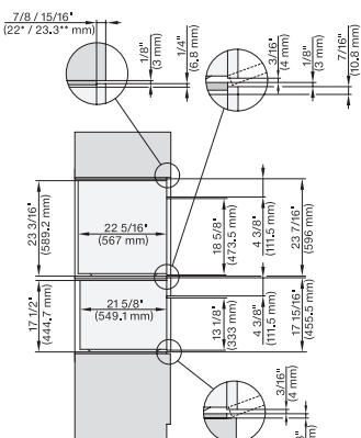
DGC 6x6x (AM)+EBA 6808, H 6x00+EBA 6808, DGC 786x, EBA78x8, H7xxx Combi, Install. drawing, Flush inset, Flush inset, NA 7/8" – 22" mm – Glas, 15/16" – 23.3" mm – Edelstahl
