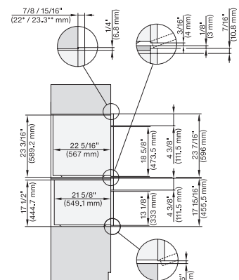
DGC6x6x(AM) + EBA6808, H6x00+EBA6808, DGC786x+EBA7868, H7x40BM+EBA7848, Combi, Installation drawing,Proud,Flush inset,NA 7/8" – 22" mm – Glas, 15/16" – 23.3" mm – Edelstahl
