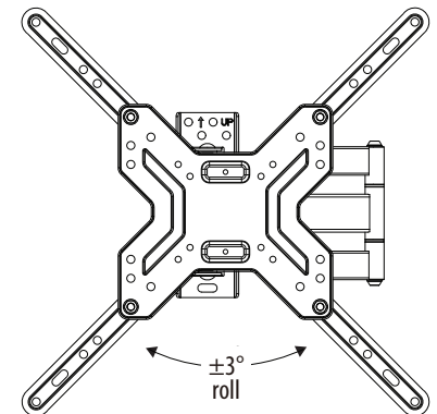
FRONT VIEW – ROLL
