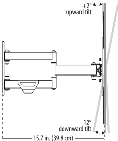
SIDE VIEW – EXTENSION/TILT
