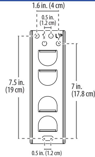
WALL PLATE
