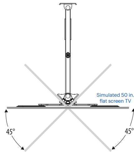
TOP VIEW – SWIVEL
