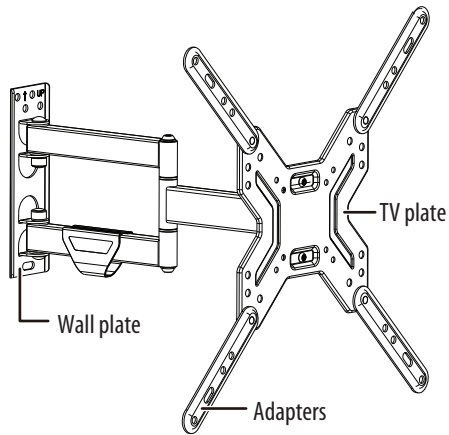
FULLY ASSEMBLED 3-D
