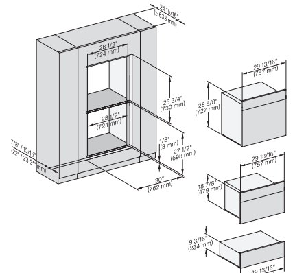
H 6x80 BP, H 6x70 BM, ESW 6x85, H 6x80-2BP, H2x80BP, H7xx0BP/BM/BPX, ESW7x70, EVS7670 Flush inset, NA
