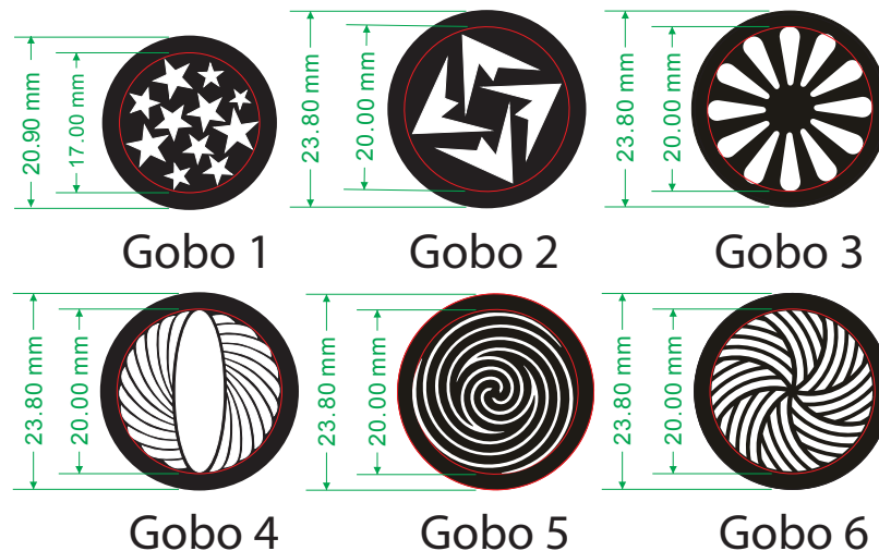
Gobo Wheel 2
