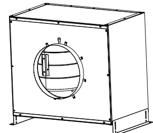
Inline Blower (ZXR610 Single, ZXR1220 Dual)
