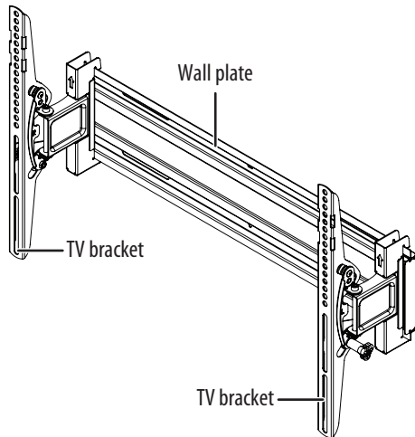
FULLY ASSEMBLED 3-D
