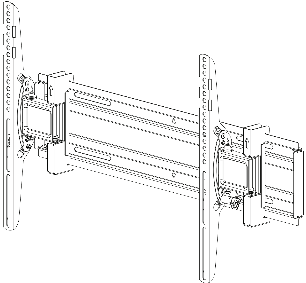
FULLY ASSEMBLED
