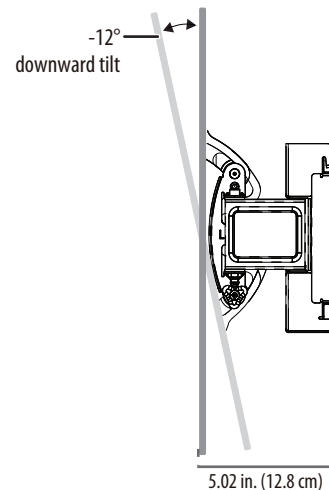
SIDE VIEW – EXTENDED/TILT
