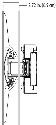
SIDE VIEW – RETRACTED
