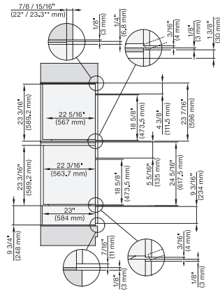
DGC786x+EBA7868, DGC7x8x, ESW7x80, EVS7670, side view, 30 Zoll, Flush inset, combi, XXL
