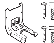
Anti-tip bracket kit
