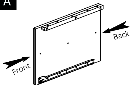
SIDE QTY 1 PAIR
