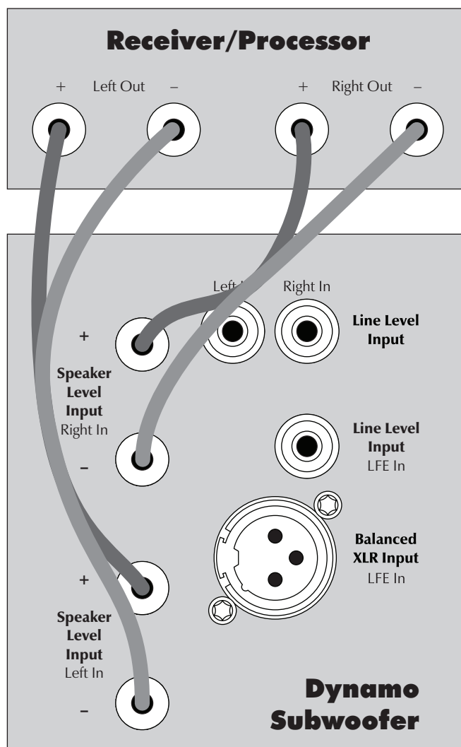
Figure 20. Signal connection for speaker level inputs.
