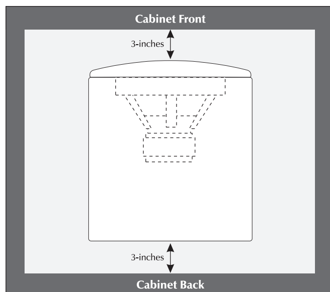
Figure 24. Placing the subwoofer in a cabinet requires a minimum of three inches of open space on the front and back.
