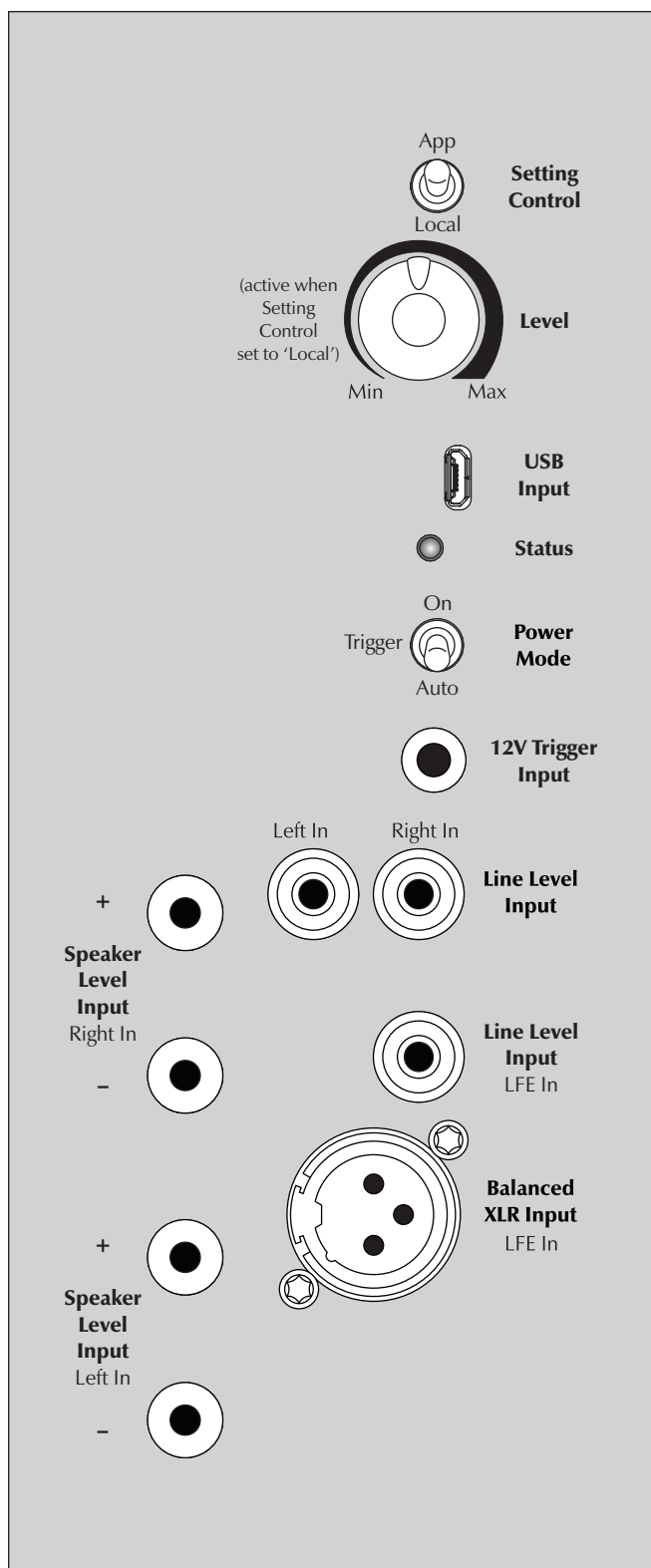
Figure 1. Controls and connections. Connection options vary by model.
