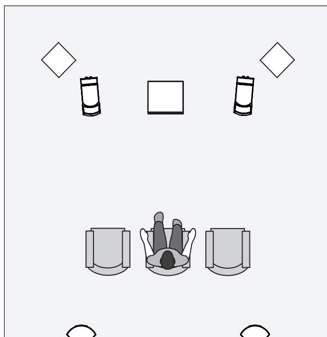
Figure 23. MartinLogan subwoofers as the LFE channels, MartinLogan speakers as front, center, and surround (effects) channels. Note the corner placement of the subwoofers at the front of the listening room.
