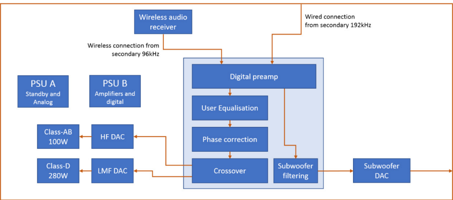
Figure 45 - Block diagram of Secondary Electronics
