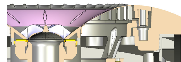
Figure 39 Cross section of complete Uni-Q driver and trim ring
