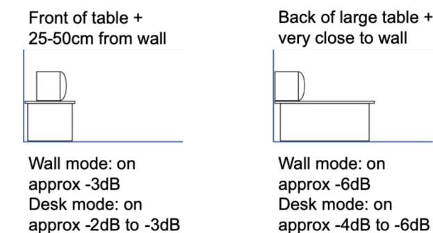
Figure 50 Recommended combined wall & desk mode settings
