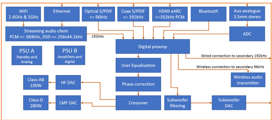
Figure 44 - Block diagram of Primary Electronics
