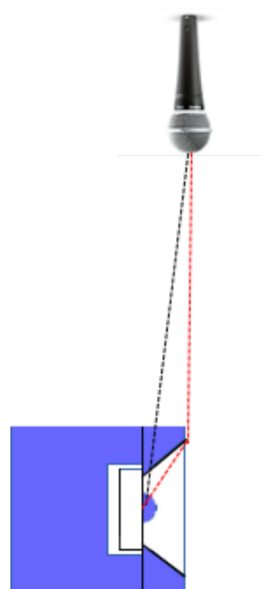
Figure 54 Conventional speaker, mic. horizontally off axis.
