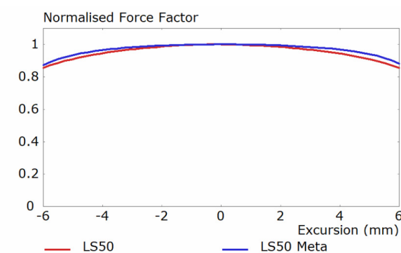
Figure 22 Comparison of bass/midrange force factor
