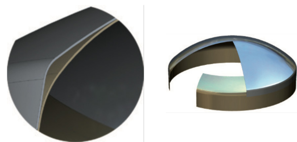
Figure 33 3D CAD sectional views of the tweeter dome and extended former that meet to form a triangular stiffening member at the dome edge
