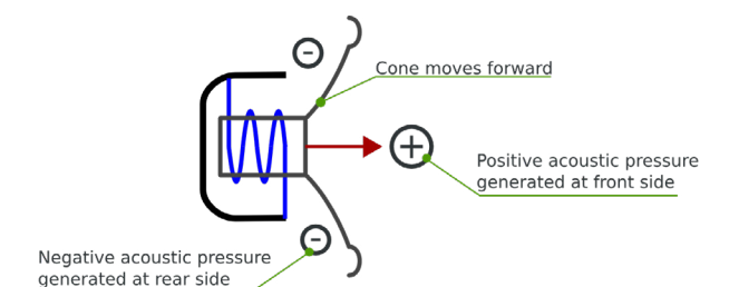
Figure 2 - Generic driver
