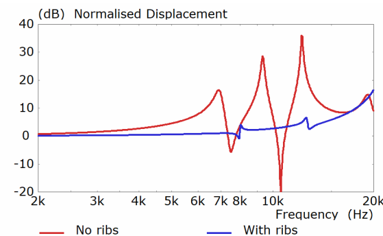
Figure 13 Simulated displacement of tangerine waveguide
