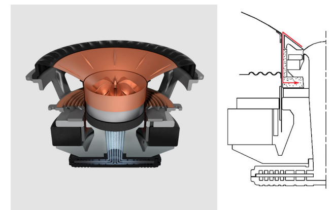
Figure 14 Uni-Q driver with damped, optimised gap
