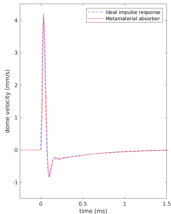
Figure 8 Impulse response of tweeter dome velocity (red), overlaid with ideal response (dotted blue)
