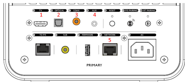
Figure 43 Primary Speaker Inputs
