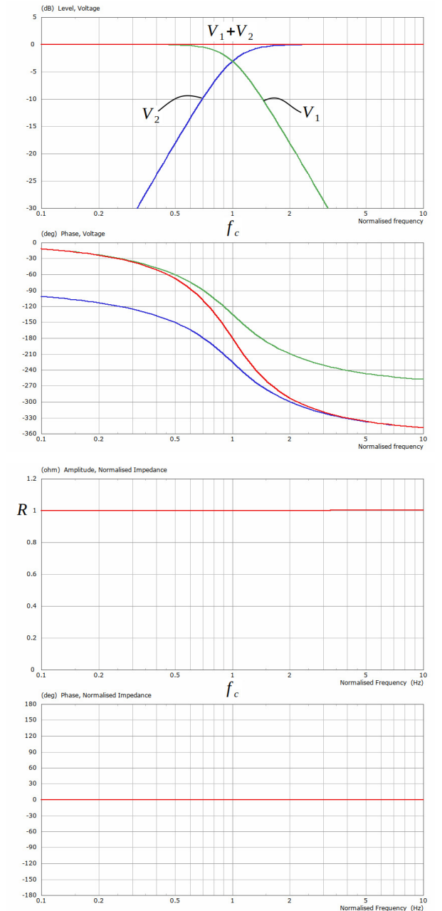
Figure 7 Top: Amplitude and Phase responses of transfer functions V_1 (green), V_2 (blue) and V_1+V_2 (red). Bottom: Amplitude and Phase responses of input impedance
