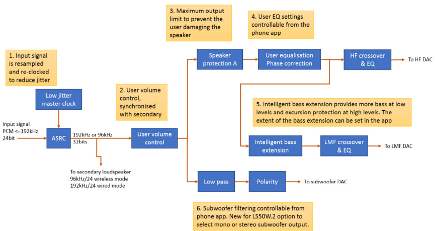
Figure 46 - DSP Details
