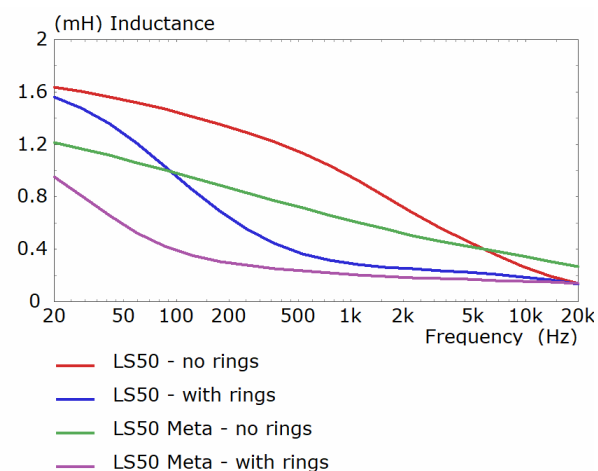
Figure 19 Bass/midrange blocked voice coil inductance against frequency.
