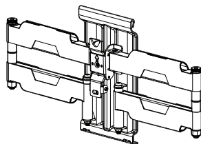
11 Arm assembly (1)
