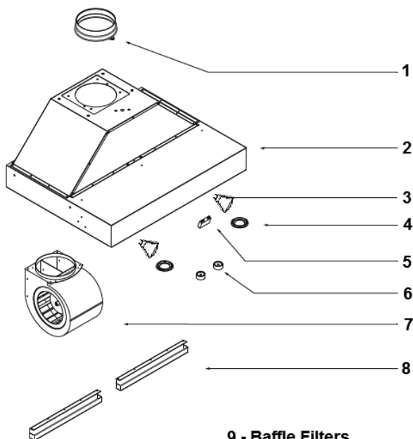
9 - Baffle Filters
