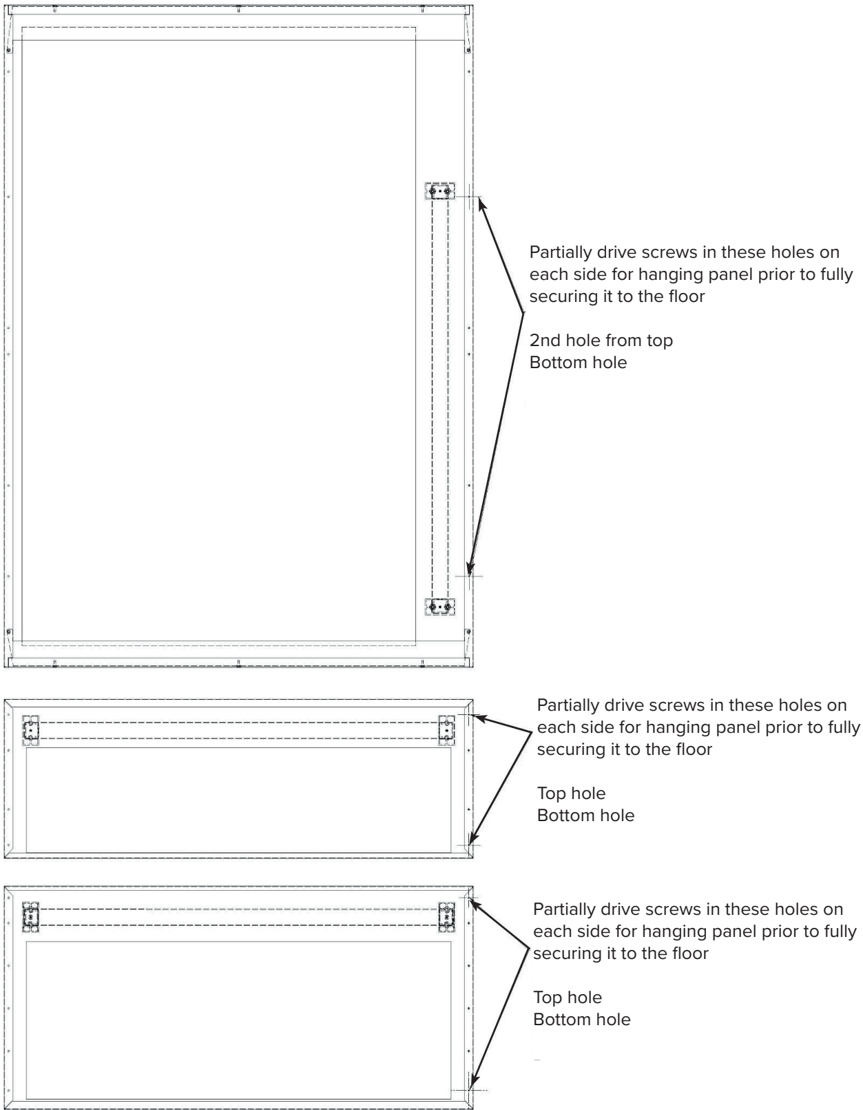
REAR VIEW
