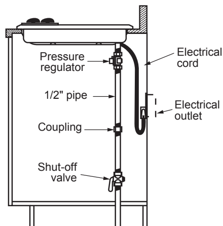
Gas Connection
