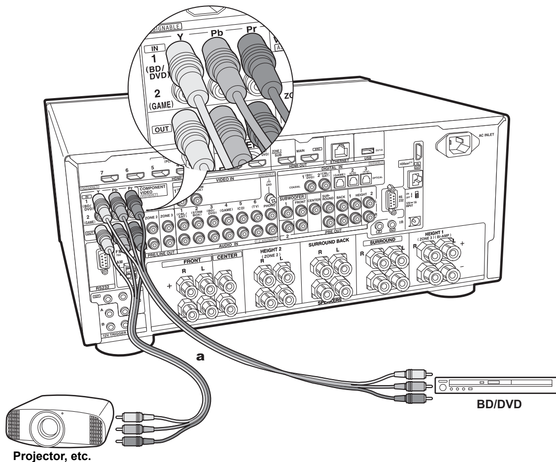
a Component Video Cable
