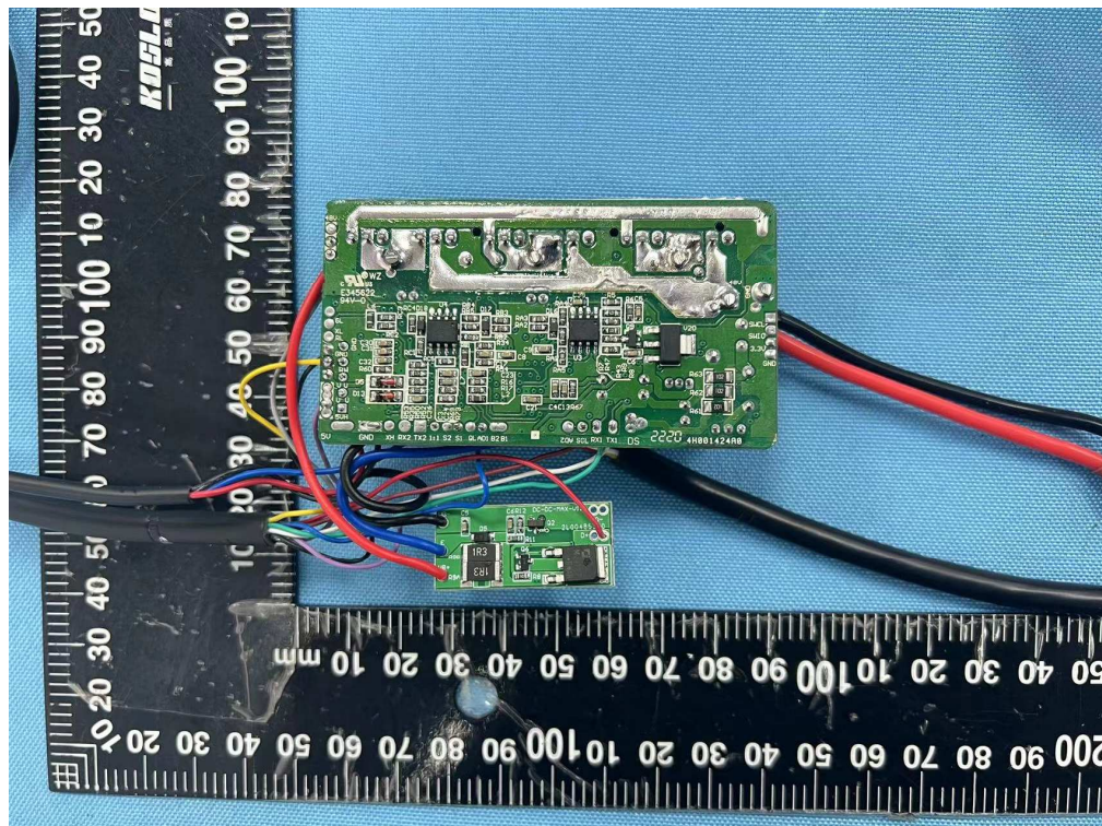
Figure 16.: Controller view
