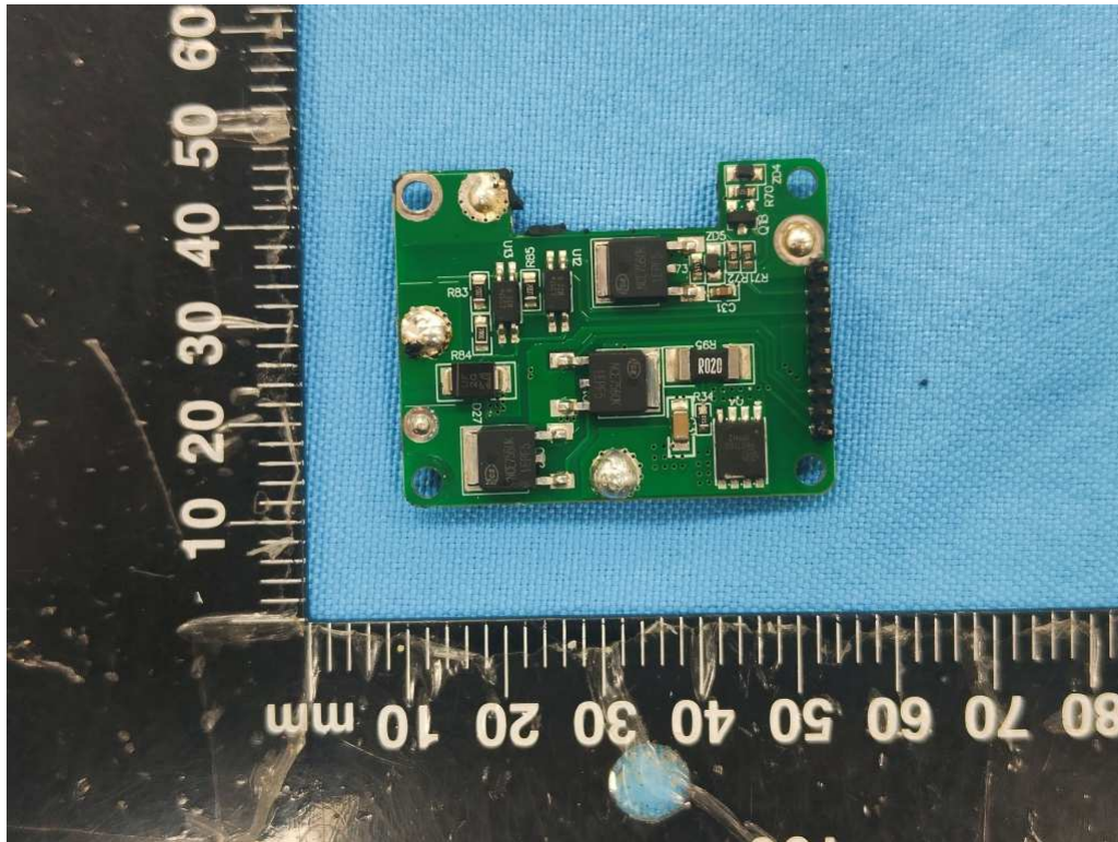
Picture 34. Protection board view-5
