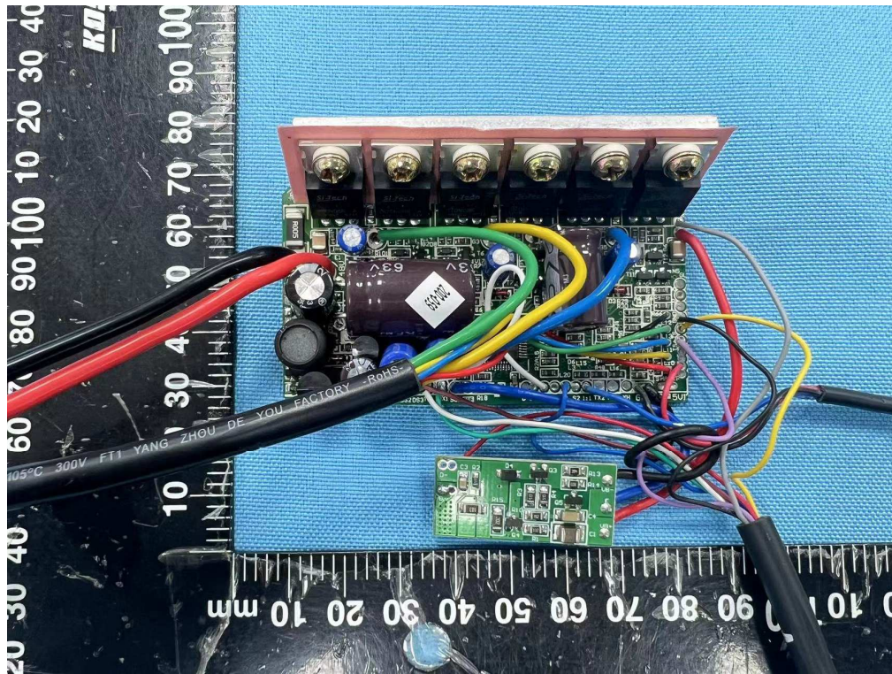
Figure 15.: Controller view
