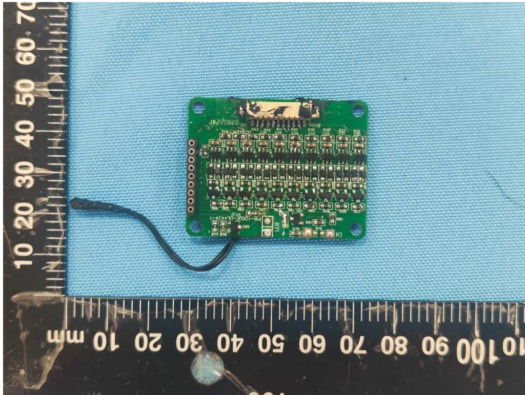
Picture 32. Protection board view-3
