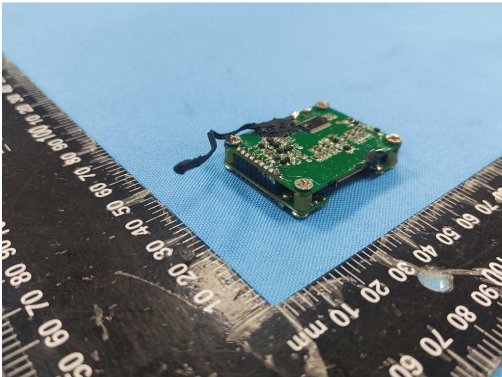
Picture 31. Protection board view-2
