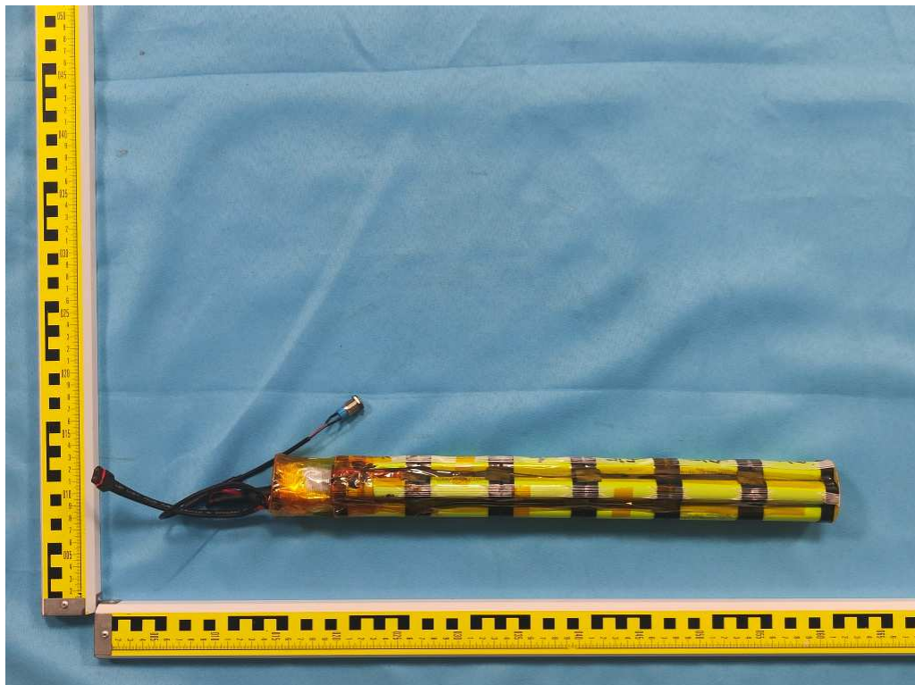
Picture 25. Inner view-4 of battery
