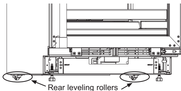
Rear leveling roller adjustment screw
