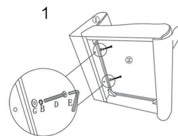
(G*2) M8*Φ22*2
