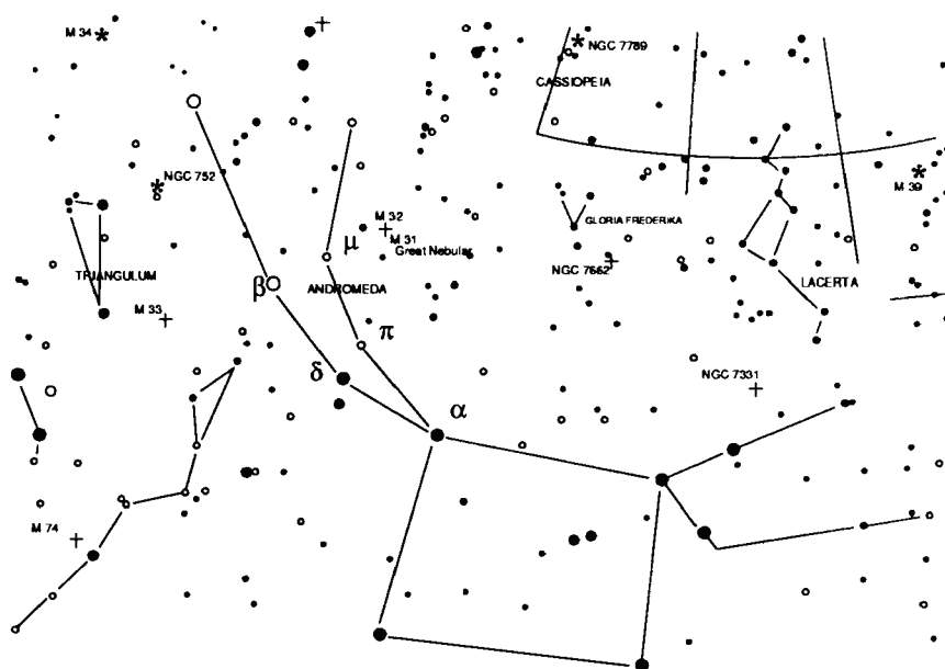
Fig. 16 Andromeda Galaxy
