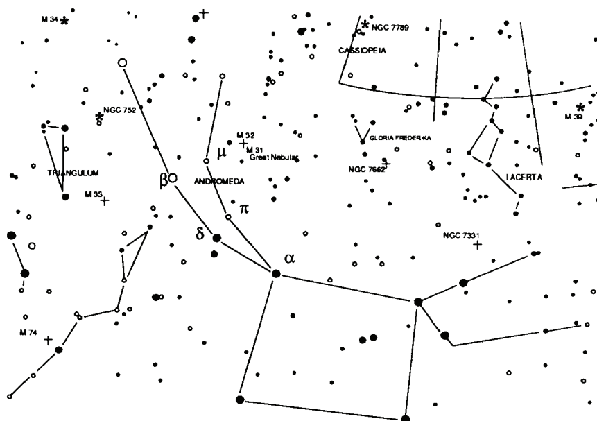
Fig. 16 Galassia Andromeda
