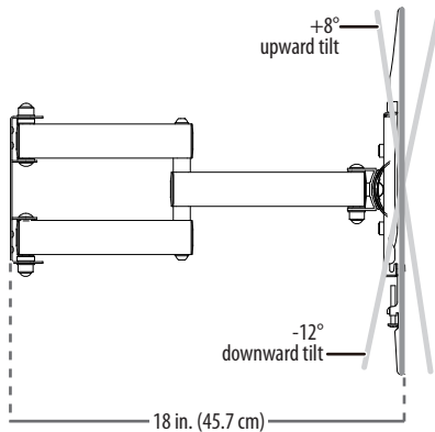
SIDE VIEW – EXTENDED/TILT
