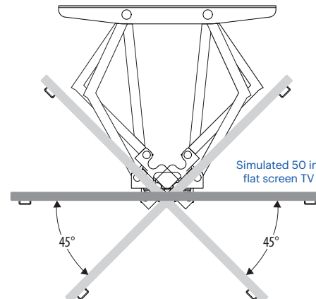
TOP VIEW – SWIVEL
