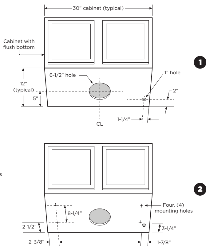
Cabinet or soffit with flush bottom
