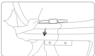
①Take down the license plate. ②Tow the camera power line into the car though the interstices of the car. ③Install the camera onto the license plate, fix it with the spared screws.
