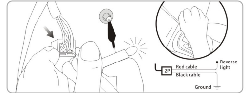
⑤Black clamp connects to any iron part of car. Use the red pen to test every power line from the reverse light until the LED light is on. Then you can ensure that this is the power line.
