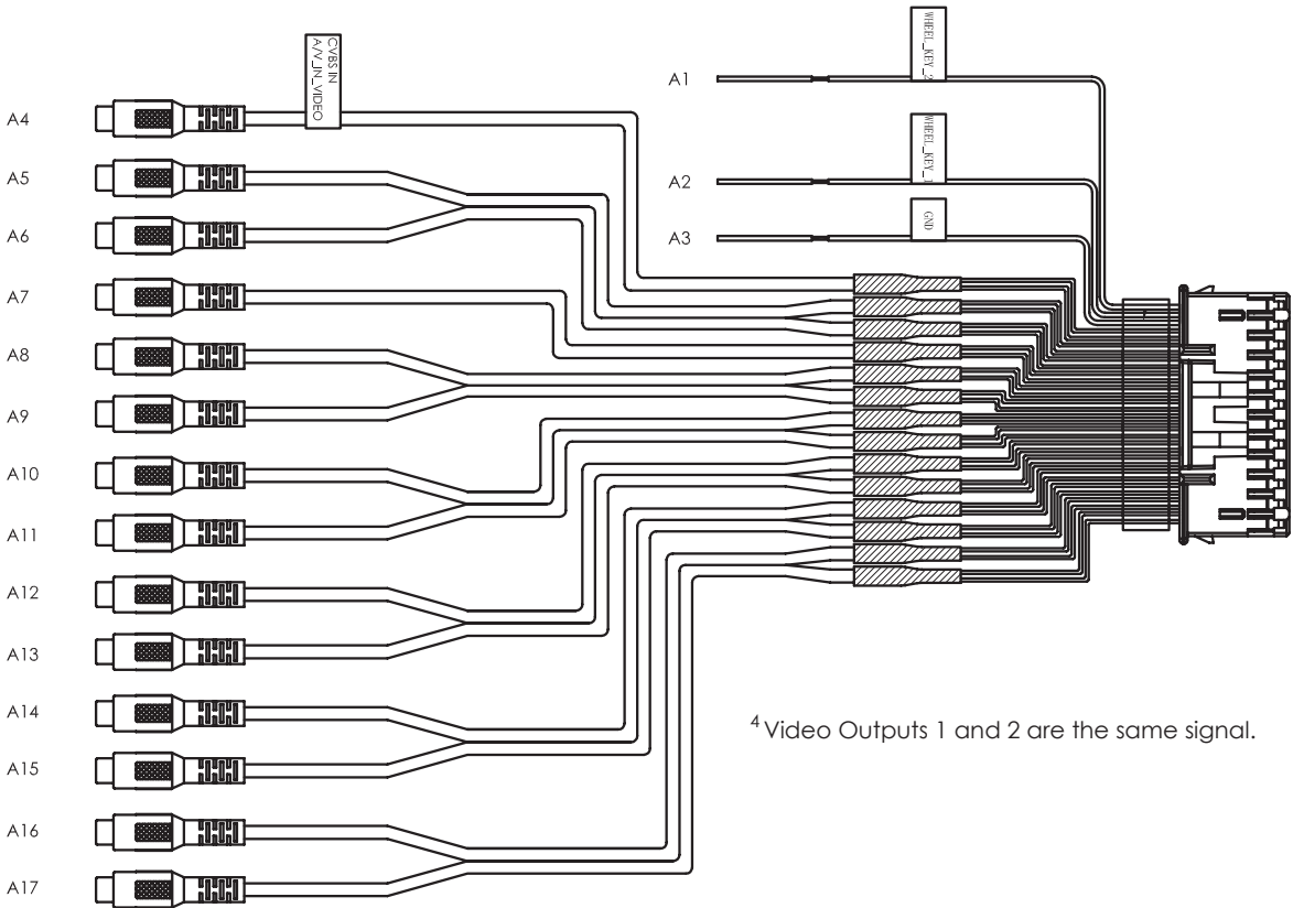
Connector View is pin side
