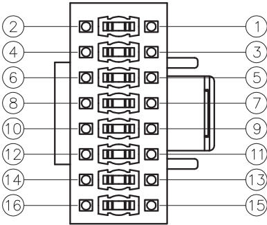
Connector View is pin side
