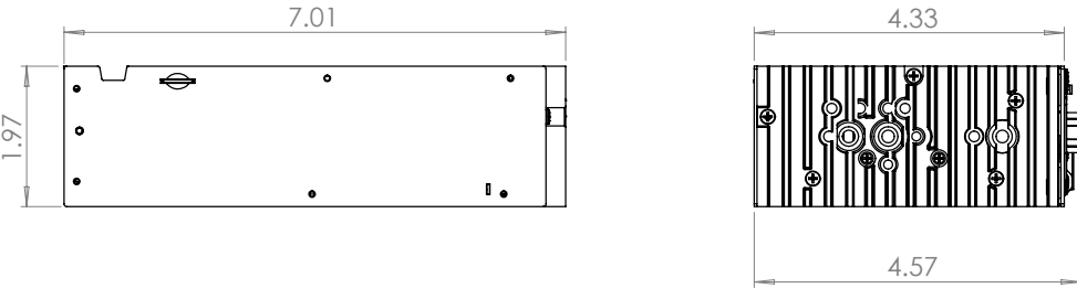
DIMENSIONS ARE IN INCHES
