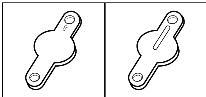
Make sure arrow on front of shim points up
