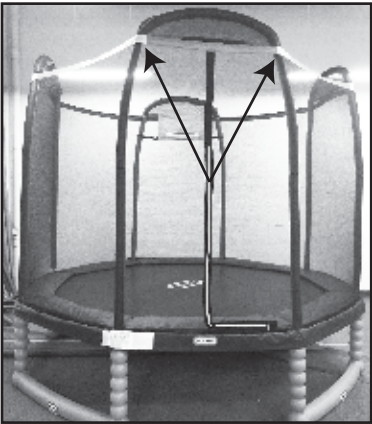
Adjust netting arch pocket to fit by pulling down the two ends of the pocket. Pockets should be secured on each of the four arches.
