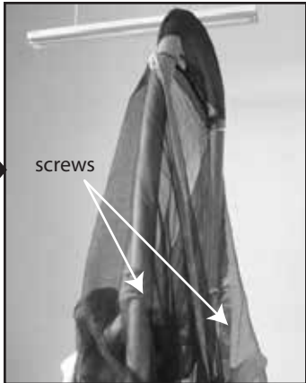
Connect curved frame tubes (J) and horizontal tubes into the straight frame tubes (I) and secure with two screws (M). Make sure curved frame tubes (J) with horizontal tube (H) tilt inward. Repeat for all arch assemblies.
