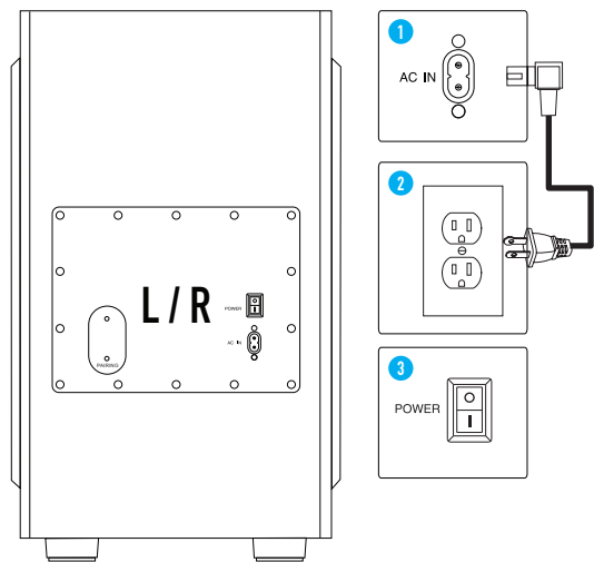
Dual-Opposing 8" Subwoofer
