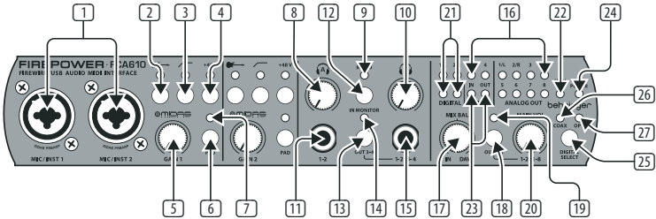
FCA610 Front
