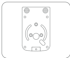
c.Mounting Plate
