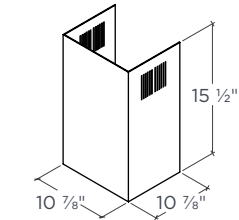
UPPER CHIMNEY COVER
