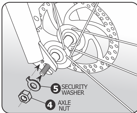
Security Washer Diagram
