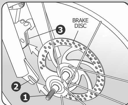
Hub Insertion Diagram
