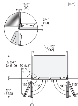
KFMC3642FD, MasterCool III, stainless steel frame, with stainless steel front, top view
