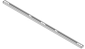
6 Center Rail (1) 35x50x1875mm
