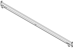
4 Side Rail (2) 100x55x2040mm
