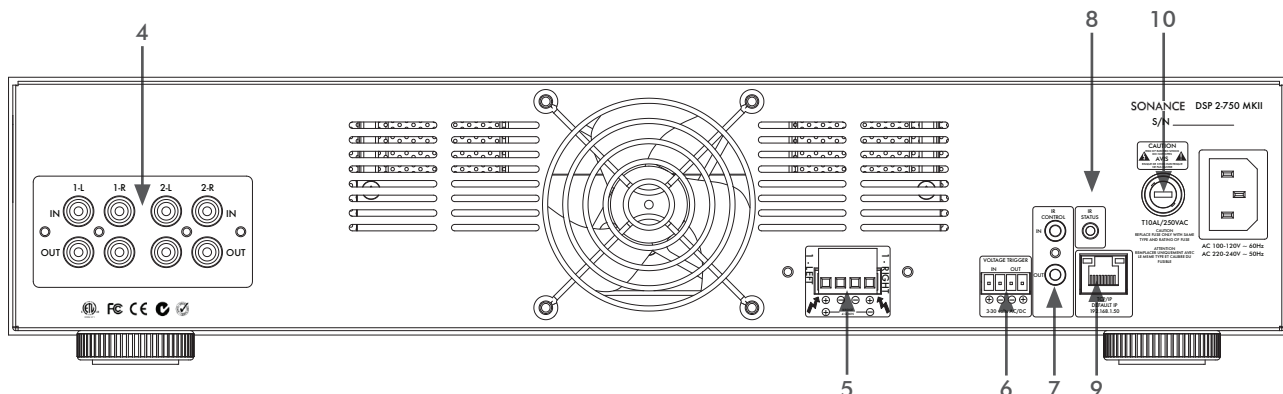
Figure 3: Sonamp DSP 2-750 MKII Multi-Channel Power Amplifier Rear Panel
