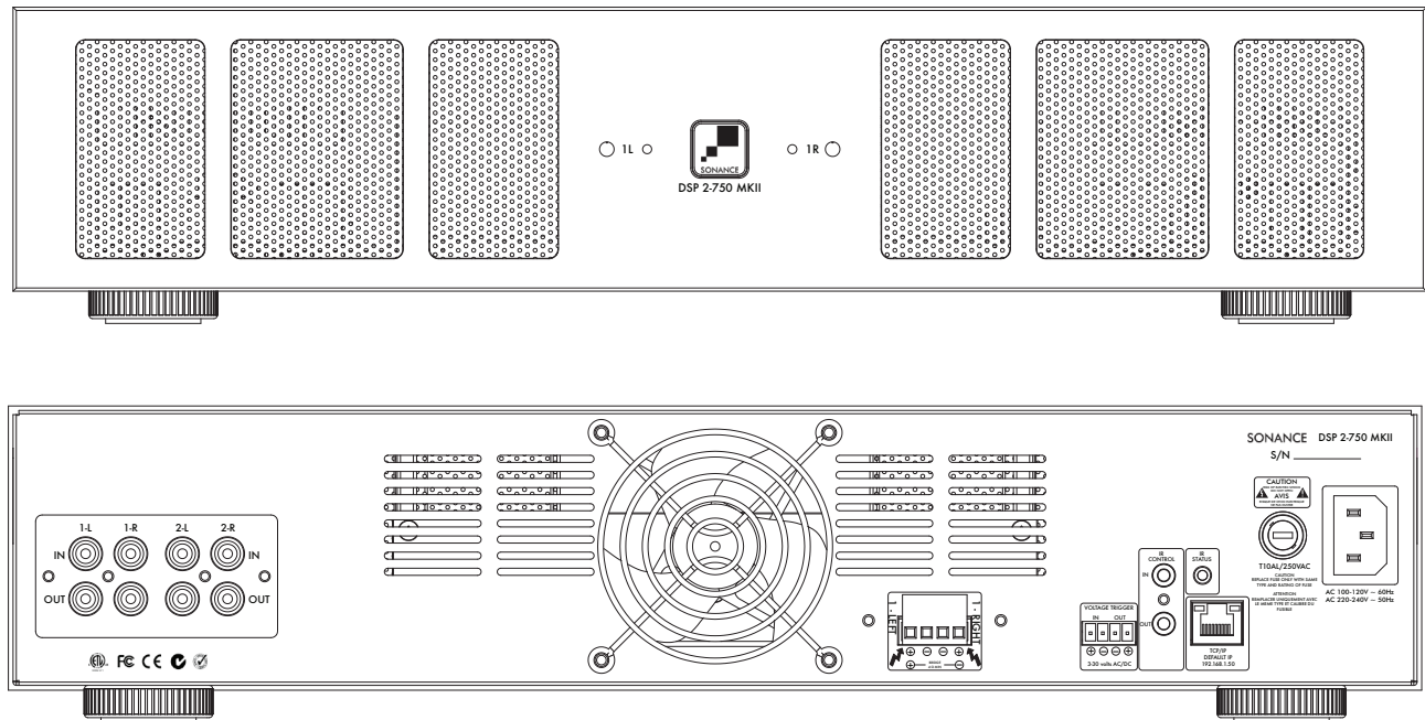
Figure 1: Sonamp DSP 2-750 MKII Multi-Channel Power Amplifier
