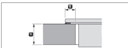
Fig. 11.7 Overlay dimensions for surface mounting
