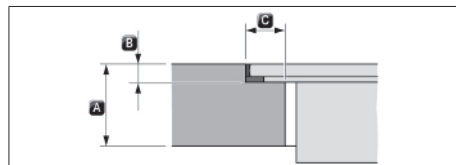
Fig. 11.5 Rebate dimensions for flush installation
