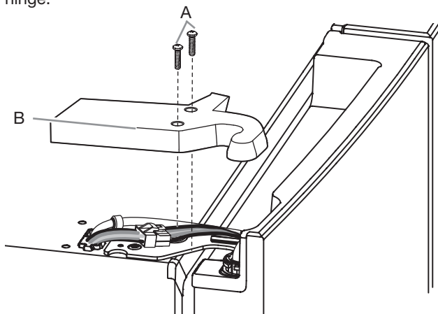
A. Top hinge cover screw
