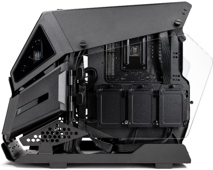
CABLE MANAGEMENT
