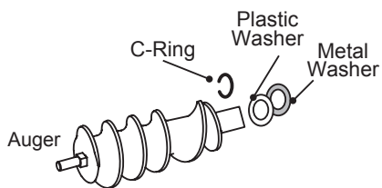
5 Auger Assembly
