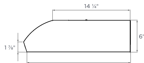
SIDE
