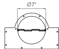
TOP ROUND EXHAUST ADAPTER
