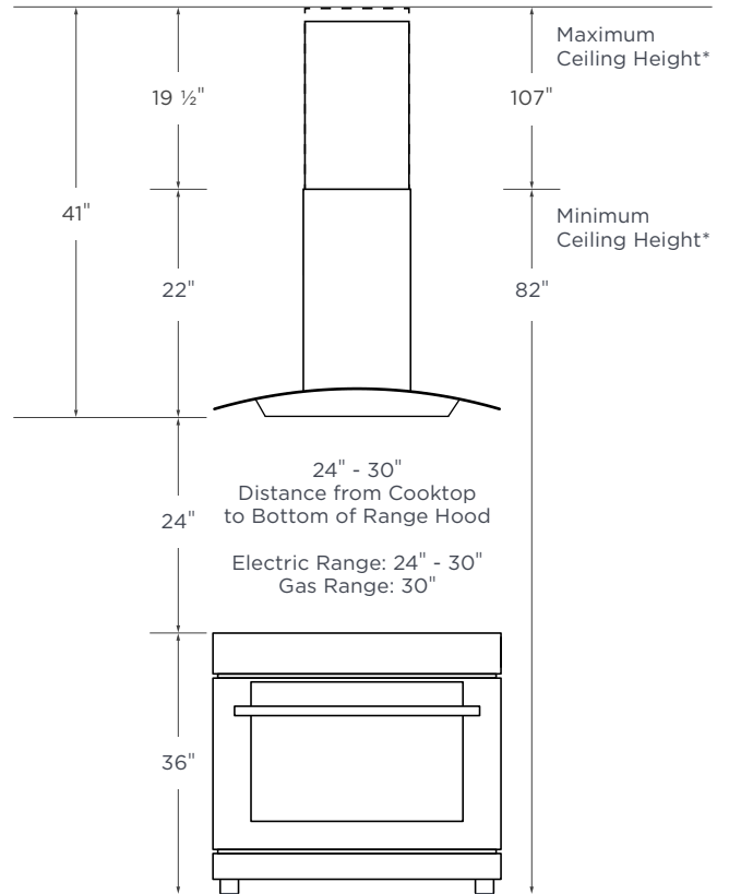
CHIMNEY EXTENSION (CHE007, SOLD SEPARATELY*)
