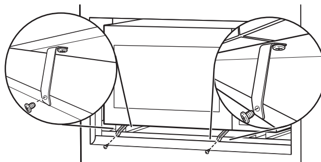
Bottom Duct Attachment Brackets
