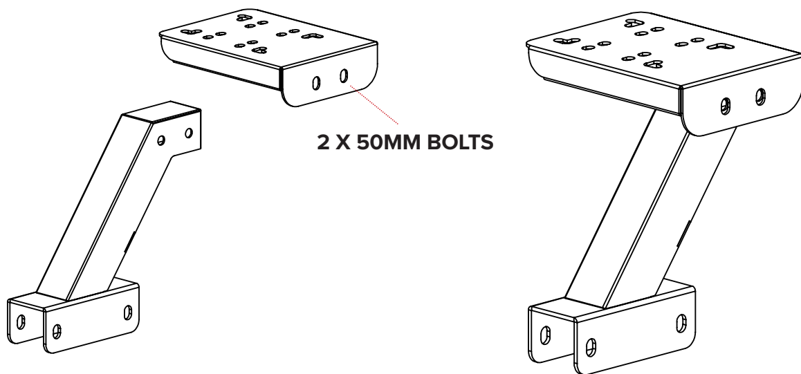
Right hand side shifter
