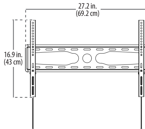
FULLY ASSEMBLED FLAT
