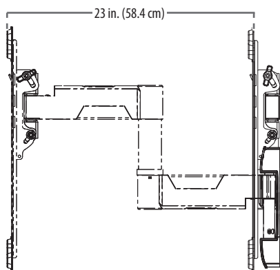
SIDE VIEW - EXTENDED
