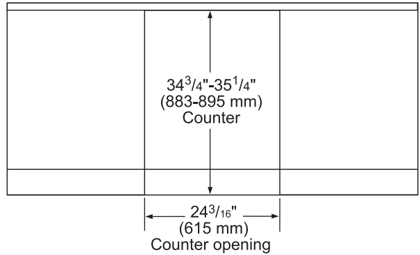
Frontal view
