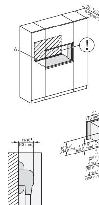
installation 30 inch Flush inset DGC30 XL, installation drawing, NA
