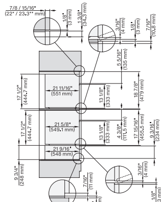
H 6x70 BM, H 6x00 BM + EBA 6808, ESW 6x85, DGC7x7x, EBA7848, H7xxx, ESW7x70 Combi, installation drawing, Flush inset, NA
