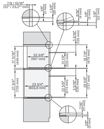
DGC7x7x(X), H7x8x(X)BP, side view, 30 Zoll, Flush inset, combi, XL, 650
