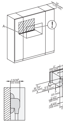
installation 30 inch Proud wide front DGC30 XL, installation drawing, NA
