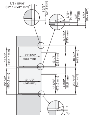
H6560B + EBA6808, H6x60BP + EBA6808, H6x70BM, DGC7xxx+EBA7484, H7xxx+EBA7868, Combi, Installation drawing, Proud, NA
